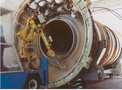
Surface preparation on a booster rocket
