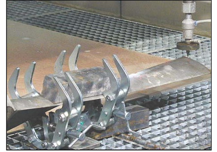
Reconditioning turbine blades
